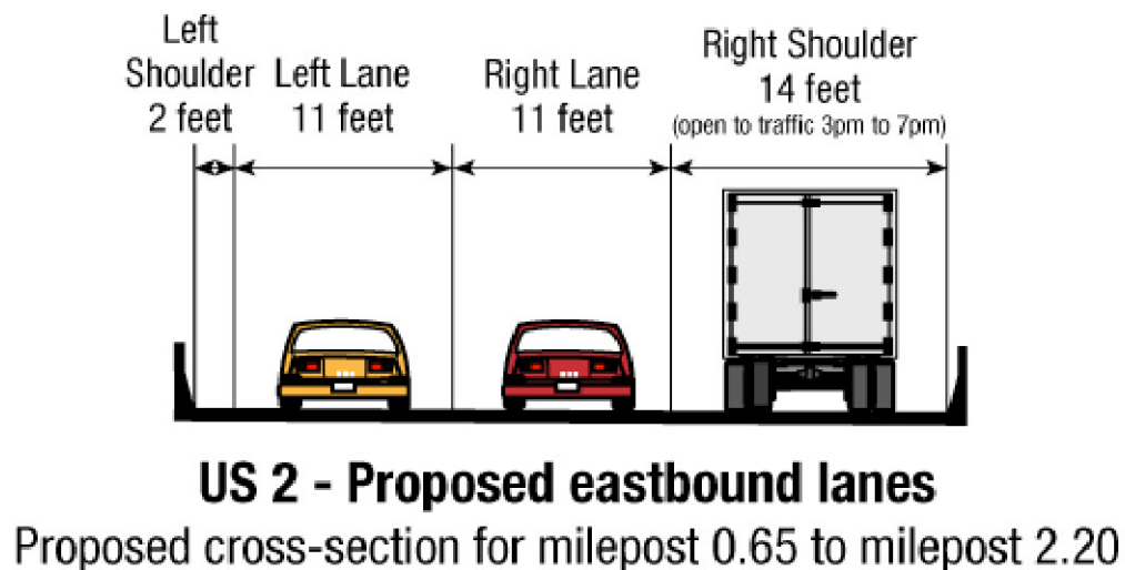
Figure 49. Illustration. US 2 Cross-Section for Shoulder Use—Everett, Washington. (55)
